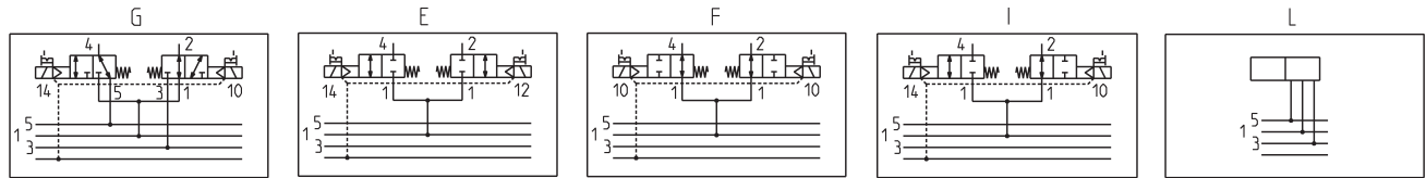
G = 1 x 3/2-way NC + 1 x 3/2-way NO
