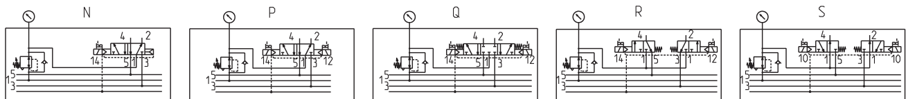
N = 5/2-way, Monostable
