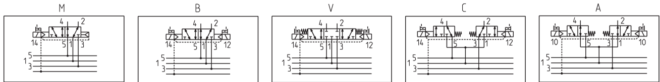
M = 5/2-way, Monostable
