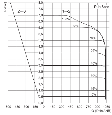
Typical curve for version PME1M4-EG...
